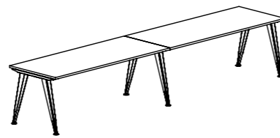
compact desk "A" | compacto "A" mesa compacto "A" | table compact "A" 1400 | 1600 | 1800 x 1415 x 740
