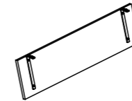
modesty panel | painel frontal faldón frontal | voile de fond 350 | 550 | 750 | 950 | 1150 | 1350 | 1550 x 300
