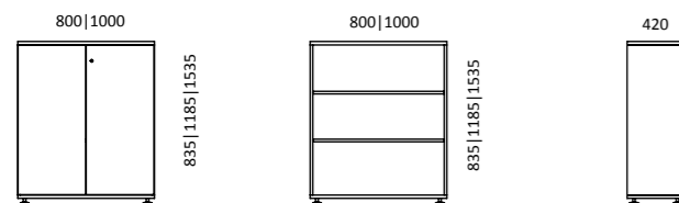
melamine cabinet | armário melamina | armario melamina | armoire melamine
