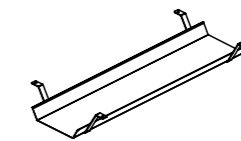
single cable channel | calha simples caja simples | goulotte simple 400 | 600 | 800 | 1000 | 1200 | 1400 | 1600 x 130 x 140
