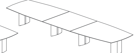
C5400xL1500xA720
